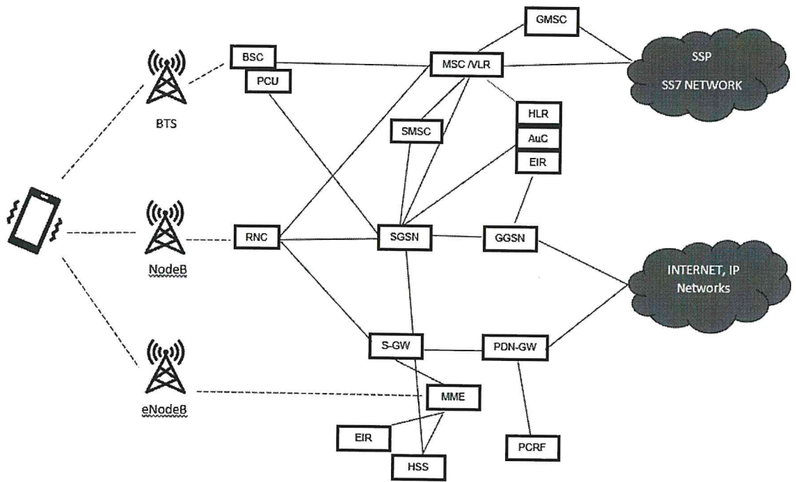
Figure 1: GSM to LTE Cellular Communication Network Architecture
